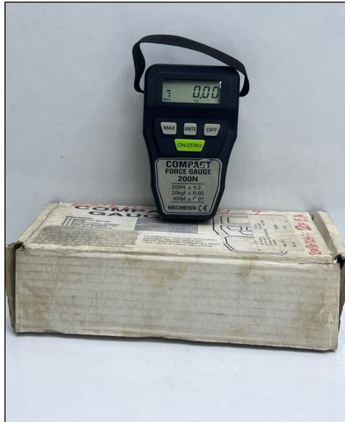
Dinamometre (Compact Force Gauge 200N)
